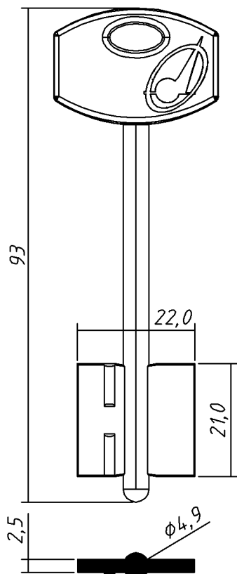
HP0 MASH 91-25PL
